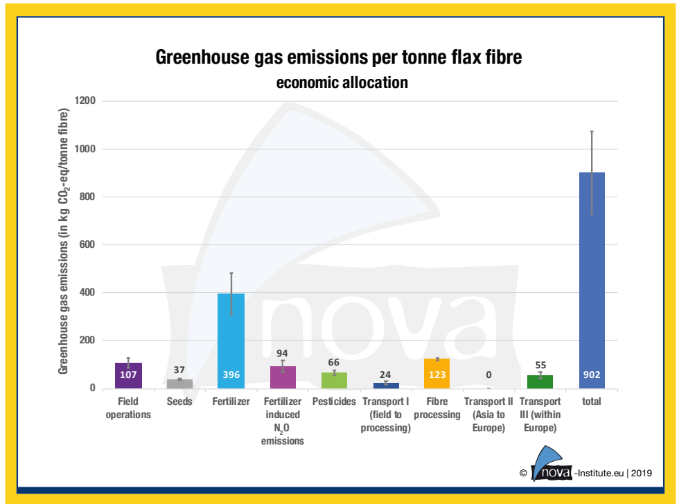
Figure 7b: Greenhouse gas emissions of 1 tonne flax fibre from the cultivation in Europe to the factory gate of the non-woven producer in Germany (nova 2019)
