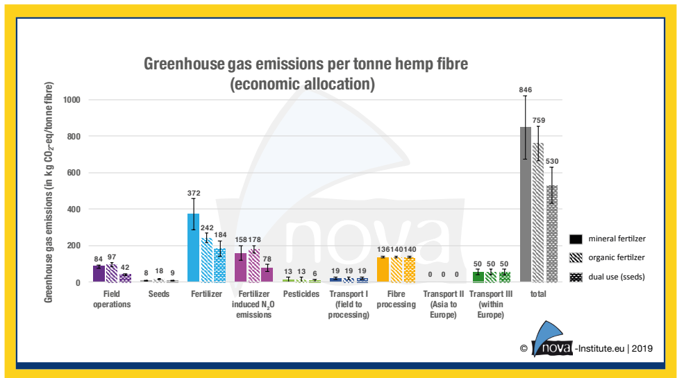
Figure 9: Greenhouse gas emissions of 1 tonne hemp fibre from the cultivation in Europe to the factory gate of the non-woven producer in Germany (nova 2019)
