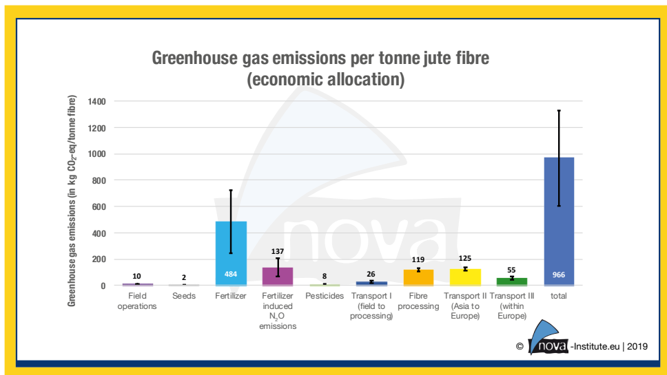
Figure 11: Greenhouse gas emissions of 1 tonne jute fibre from the cultivation in India to the factory gate of the non-woven producer in Germany (nova 2019)
