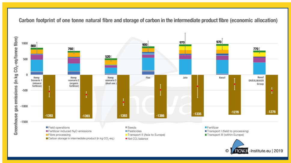
Figure 18: Overview of the greenhouse gas emissions per tonne natural fibre and carbon storage (in CO 2 -eq.) in the intermediate product fibre (flax, hemp, jute and flax) (nova 2019)
