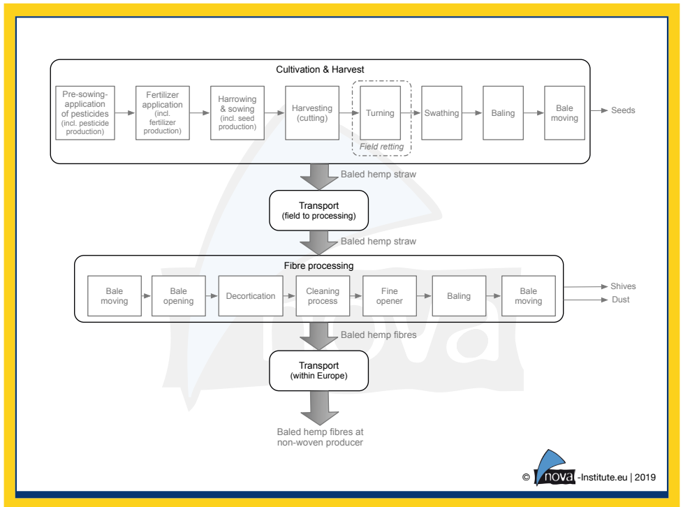
Figure 8: System boundary and process chain of the hemp fibre production (total fibre line) (nova 2019)
