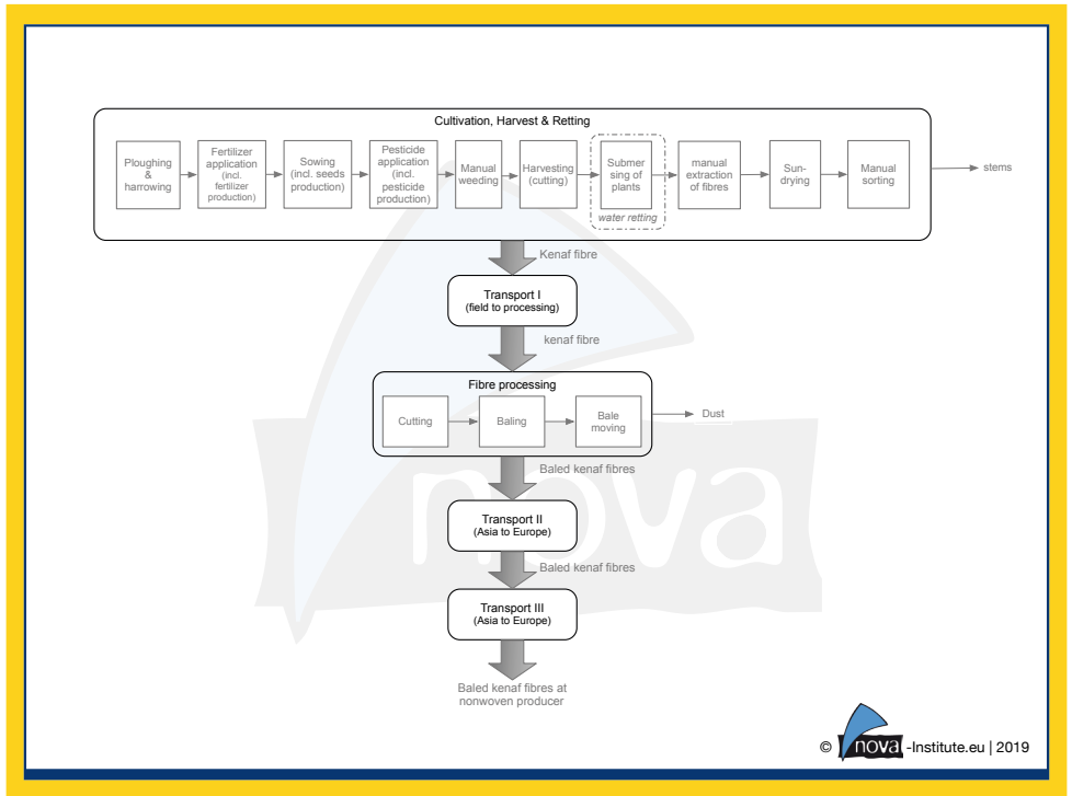
Figure 13: System boundary and process chain of the kenaf fibre production by DRÄXLMAIER Group (nova 2019)
