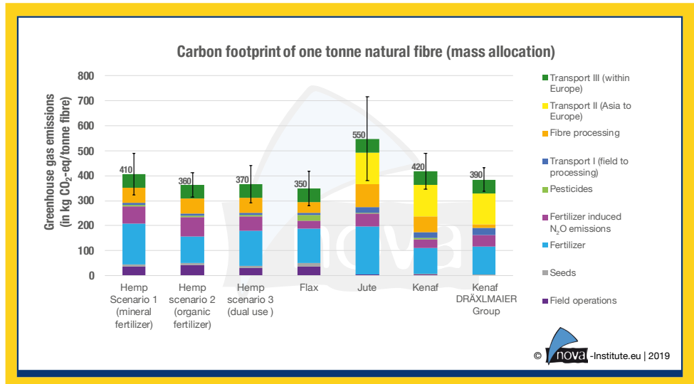
Figure 15: Overview of the greenhouse gas emissions per tonne natural fibre, using mass allocation (flax, hemp, jute and flax) (nova 2019)
