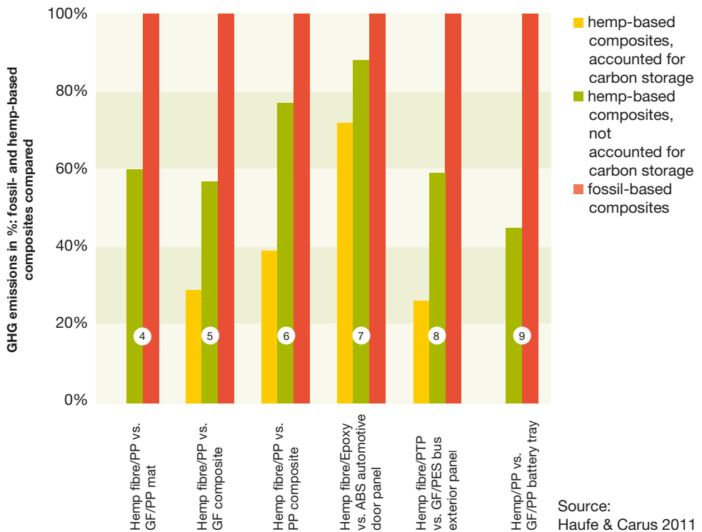
Figure 19: GHG emissions expressed in percent for the production of fossil based and hemp-based composites for a number of studies – showing the effects of biogenic carbon storage where available (Haufe & Carus 2011)
