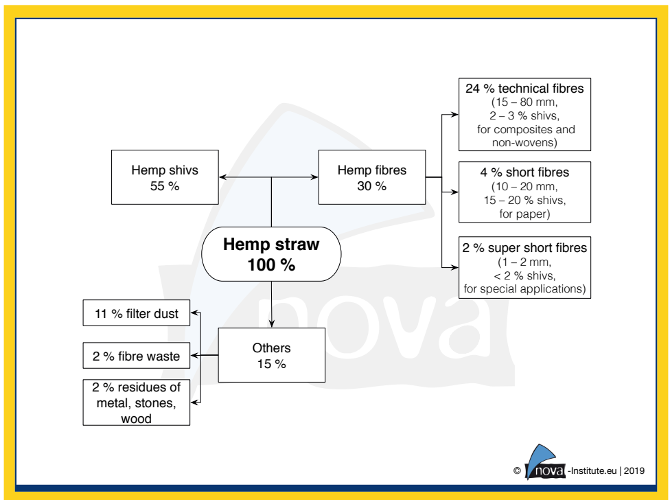
Figure 5: Typical product fractions of a total fibre line for hemp fibre production (nova 2019)
